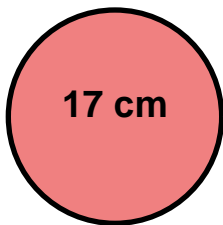
Sea level rise over next 30 years
