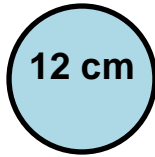
Sea level rise over last 30 years
